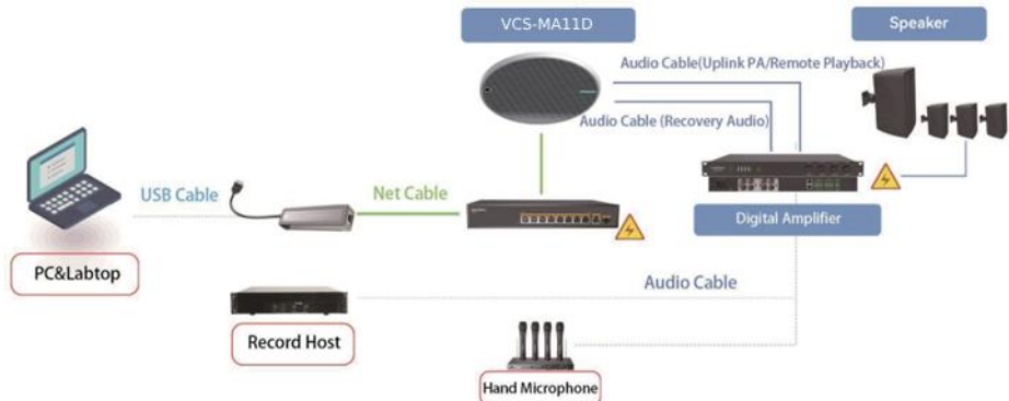
Dante digital audio topology
